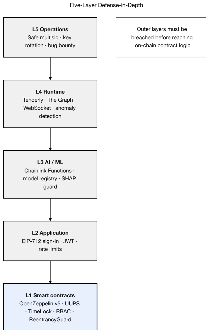
Figure 3.35: Five-layer defense-in-depth security architecture. Each layer is necessary; breaching the smart-contract layer requires defeating every layer above it. Layer 1 (smart contract): OpenZeppelin v5, UUPS, TimeLock, RBAC, ReentrancyGuard, audit suite. Layer 2 (application): EIP-712 sign-in, JWT, rate-limit. Layer 3 (AI/ML): commit-reveal oracle, model registry, SHAP, hallucination guard. Layer 4 (runtime): Tenderly, PostgreSQL event listener (Graph optional later), WebSocket dashboard, anomaly detection. Layer 5 (operations): Safe multisig, key rotation, bug-bounty.
