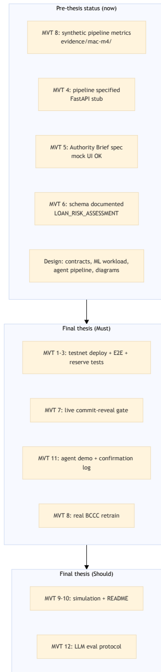
Figure 4.1: MVT deliverable status at pre-thesis submission versus final thesis targets. Pre-thesis evidence includes synthetic ML pipeline validation (MVT 8 partial), schema and workload documentation (MVT 4–6), and architectural specifications; testnet E2E deployment, live commit–reveal oracle, real BCCC retrain, and agent demo remain Phase II–IV Must items.
