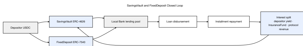
Figure 3.19: SavingsVault (ERC-4626) and FixedDeposit (ERC-7540) mobilize depositor USDC into the Local Bank lending pool; loan interest is split deterministically among depositor yield, the InsuranceFund, and protocol revenue.
