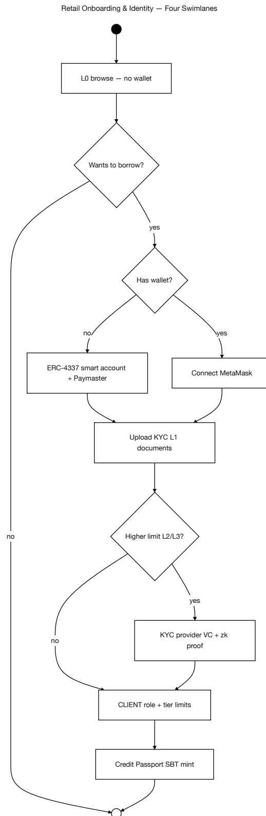
Figure 3.24: Retail onboarding and identity activity flow: progressive ladder from L0 product browse through ERC-4337 smart-account creation, document capture (L1–L3), licensed KYC provider VC issuance, zkKYC/zkAML proof generation, and on-chain CLIENT role activation with tier limits enforced.
