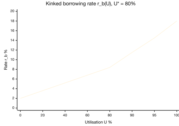
Figure 3.17: Kinked utilization-based borrowing rate r_b(U) with optimal utilization U^* = 80\% : gentle slope below the kink, steep slope above to incentivize repayment and new deposits.
