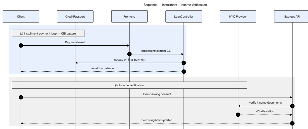
Figure 3.28: Sequence diagrams: (a) installment payment loop using the CEI pattern with SBT update on the final installment, and (b) income verification with Open-Banking pull or manual officer review.
