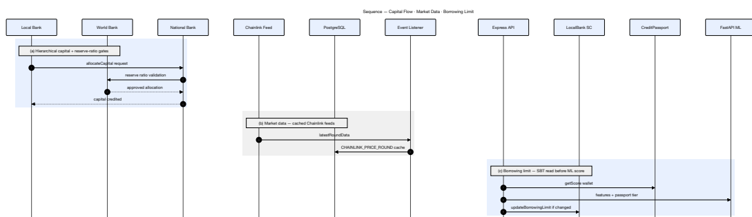
Figure 3.29: Sequence diagrams: (a) hierarchical capital flow with reserve-ratio gates at every tier, (b) market-data retrieval via cached Chainlink feeds, (c) borrowing-limit calculation reading the credit-passport SBT before ML scoring.
