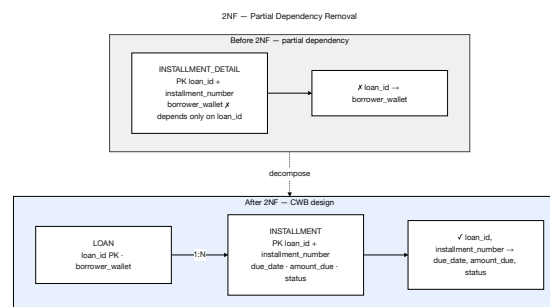
Figure 3.9: Second normal form (2NF): partial dependency on loan_id alone is removed by decomposing borrower attributes into LOAN; INSTALLMENT non-key columns depend on the full composite key.
