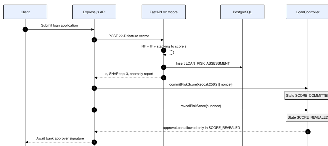
Figure 4.2: ML oracle commit-reveal gate (MVT item 7): FastAPI scoring writes an audit row, commits \text{keccak256}(s \parallel \text{nonce}) on-chain, then reveals (s, \text{nonce}) before approveLoan may succeed in SCORE_REVEALED .
