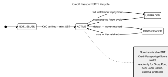
Figure 3.20: Credit Passport SBT lifecycle: non-transferable credential issued after KYC, updated on repayment, permanently downgraded (never revoked) on default, and exposed read-only via ICreditPassport.getScore() to GroupLendingPool, peer Local Banks, and external protocols.
