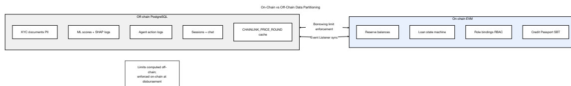
Figure 3.12: On-chain versus off-chain data partitioning: reserve balances, loan state, and role bindings on the EVM; KYC documents, agent logs, and ML scores in PostgreSQL; borrowing limits computed off-chain and enforced on-chain at disbursement.
