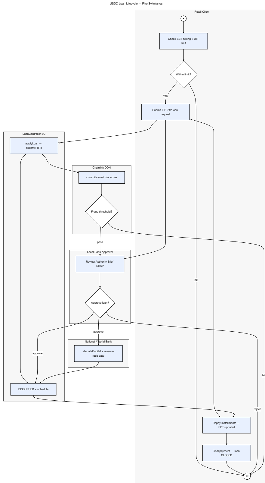
Figure 3.23: USDC loan lifecycle activity flow: five phased swimlanes from eligibility gate (SBT tier ceiling and DTI check) through origination (hierarchical allocateCapital ), oracle-mediated risk scoring (commit-reveal DON), human approver gate, to disbursement, installment servicing, and loan close.
