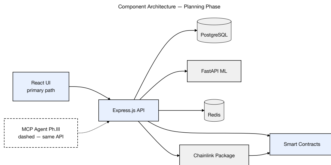
Figure 3.2: Component diagram (planning phase): React UI is the primary path; MCP agent (Phase III, dashed) shares the Express.js API; smart contracts and Chainlink integrations are specified for Phase I–IV deployment.
