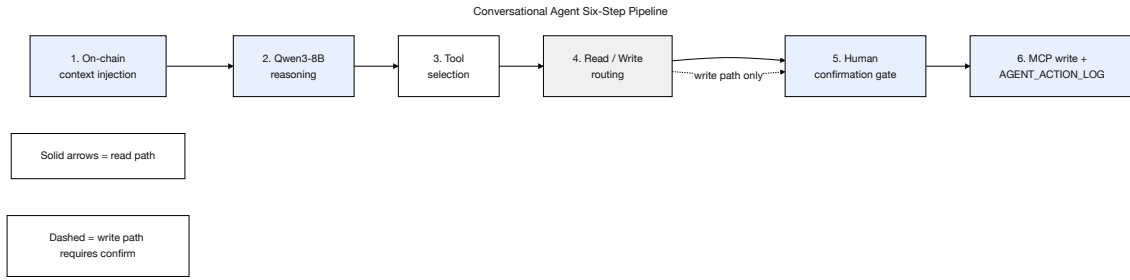
Figure 3.16: Conversational agent pipeline (Phase III Must deliverable): six-step pipeline with on-chain context injection, read/write routing, mandatory human confirmation gate, MCP write-tool execution, and AGENT_ACTION_LOG audit trail. React dashboard remains the co-primary interface.
