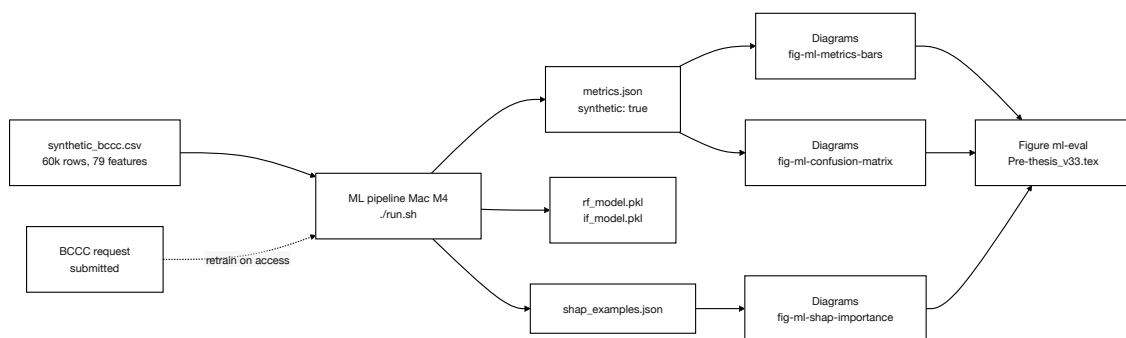
Figure 4.4: Reproducible evidence pipeline: synthetic_bccc.csv → Mac M4 run.sh → metrics.json and model artifacts → Diagrams/fig-ml-* → Figure 4.5.
