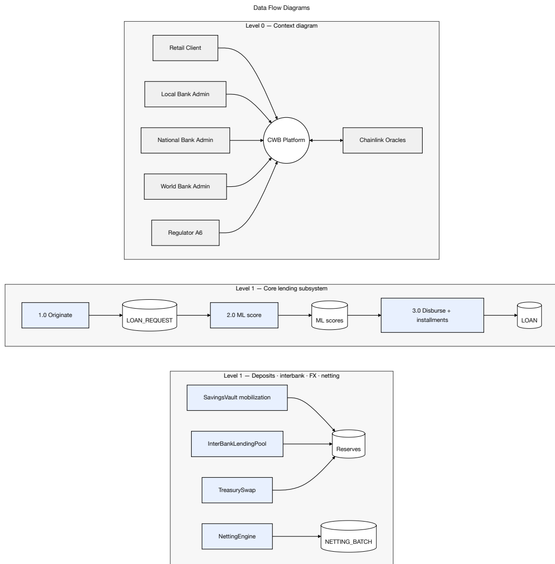
Figure 3.26: Data-flow diagrams: Level-0 context view of the Crypto World Bank platform with five external entities; Level-1 decomposition of the core lending subsystem (origination, ML scoring, disbursement, installment engine, and their data stores); and Level-1 decomposition of the deposit-mobilization, InterBankLendingPool, TreasurySwap, and NettingEngine subsystems.
