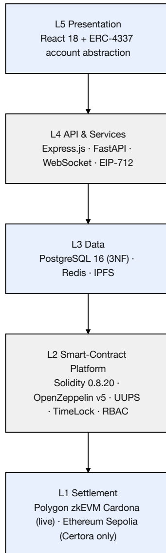
Layered Blockchain & Application Stack
