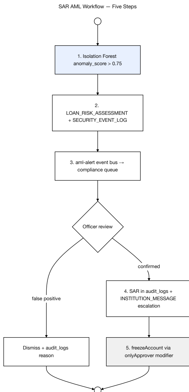
Figure 3.34: SAR and AML compliance workflow: Isolation Forest anomaly detection, compliance officer review queue, optional SAR report generation, on-chain freezeAccount via onlyApprover , and append-only audit_logs record.
