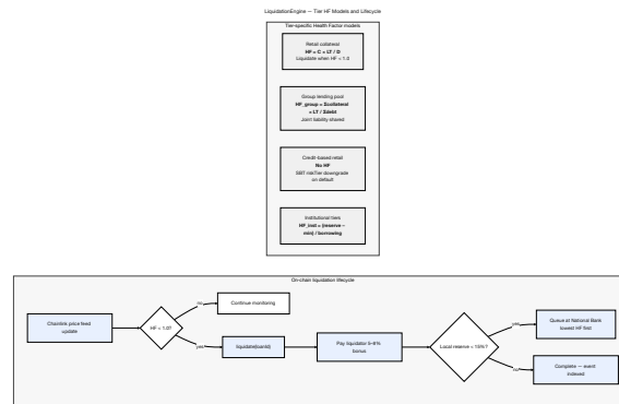
Figure 3.18: LiquidationEngine: tier-specific Health Factor models (retail collateral, group pool, credit-based SBT downgrade, institutional reserve surplus) and the on-chain liquidation lifecycle (Chainlink price update → liquidate() with 5–8% bonus → hierarchical portfolio queue when reserve ratio falls below 15%).
