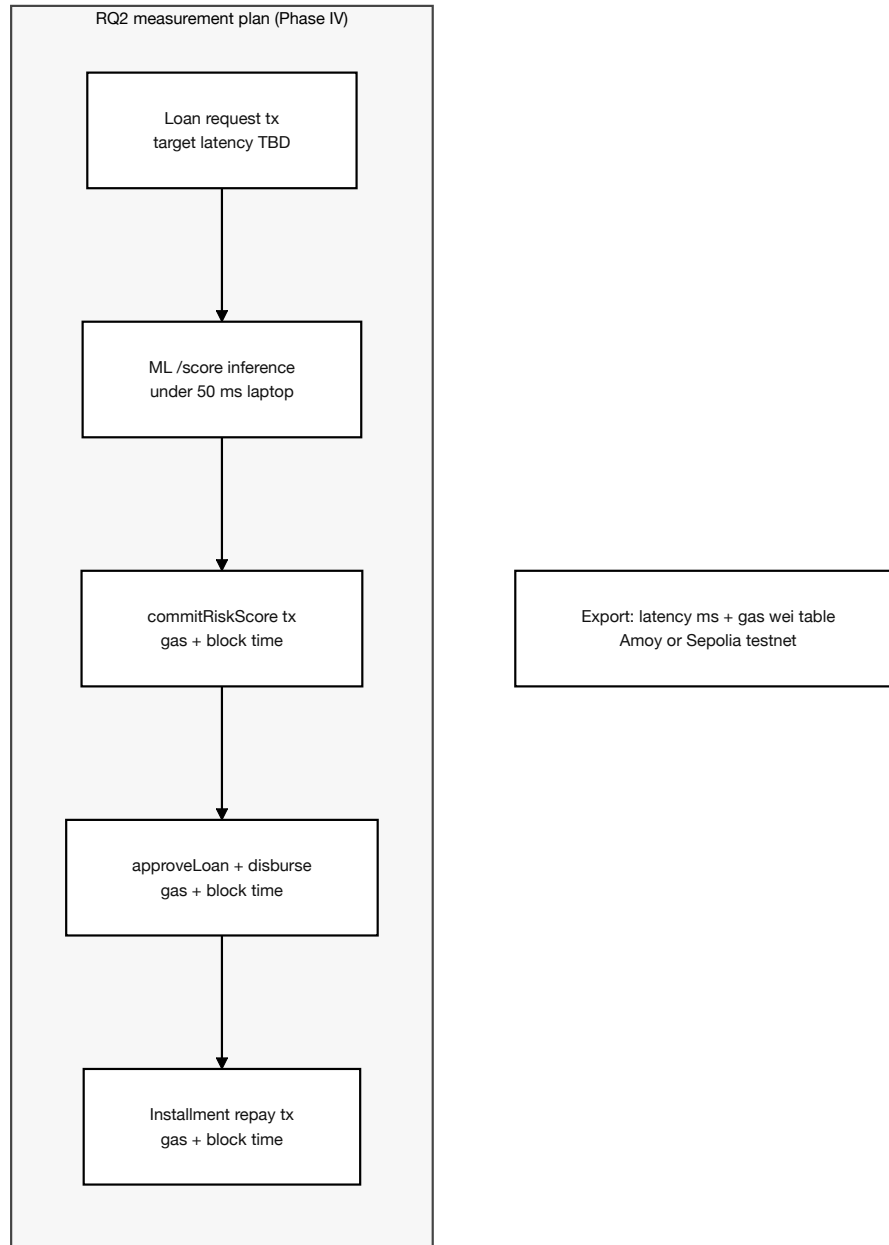
Figure 4.7: RQ2 latency and gas measurement plan (Phase IV): per-stage targets for loan request, ML inference, commit–reveal oracle transactions, disbursement, and repayment on Amoy or Sepolia testnet.
